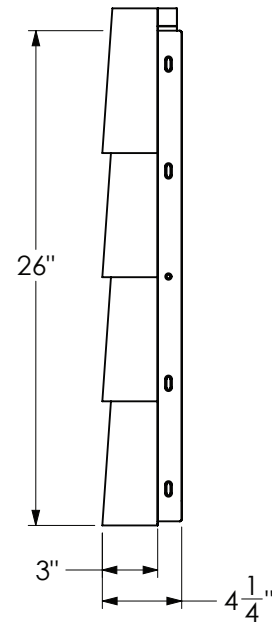
SIDE ELEVATION
