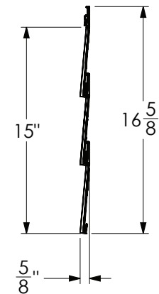
SIDE ELEVATION
